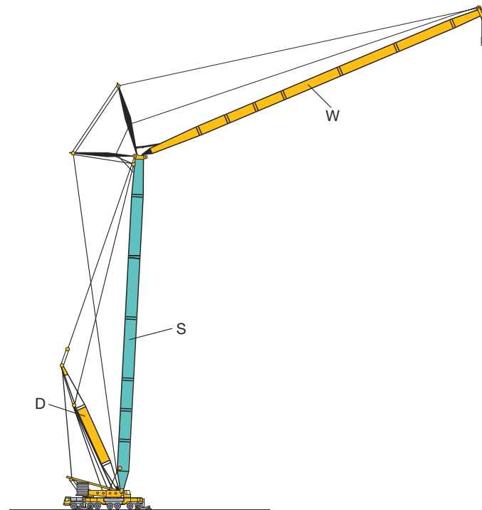
SDW 35 m – 77 m / 28 m – 84 m
