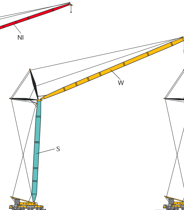
SW 28 m – 56 m / 28 m – 84 m
