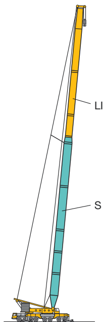
SL 21 m – 98 m
